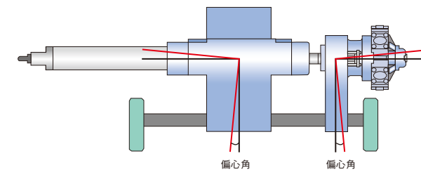
■ 一般射出機－偏心角度即為射出分力的來源。 Conventional injection machine – The eccentric angle causes injection force.
